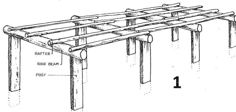
RECTANGULAR POSTS SUPPORTED ROOF BEAMS AND RAFTERS.
