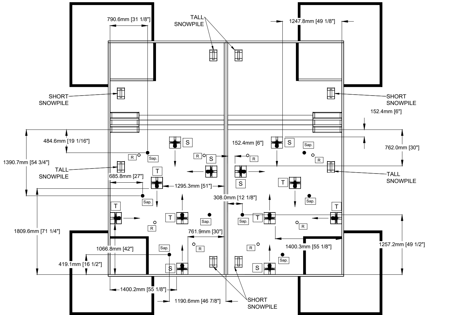
OVERALL COURT AREA (TOURNAMENT LAYOUT) SCALE = 1:50 (ON 8.5" x 11" PAPER)
