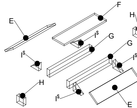
② RAMP ASSEMBLY DETAILS SCALE = N/A
