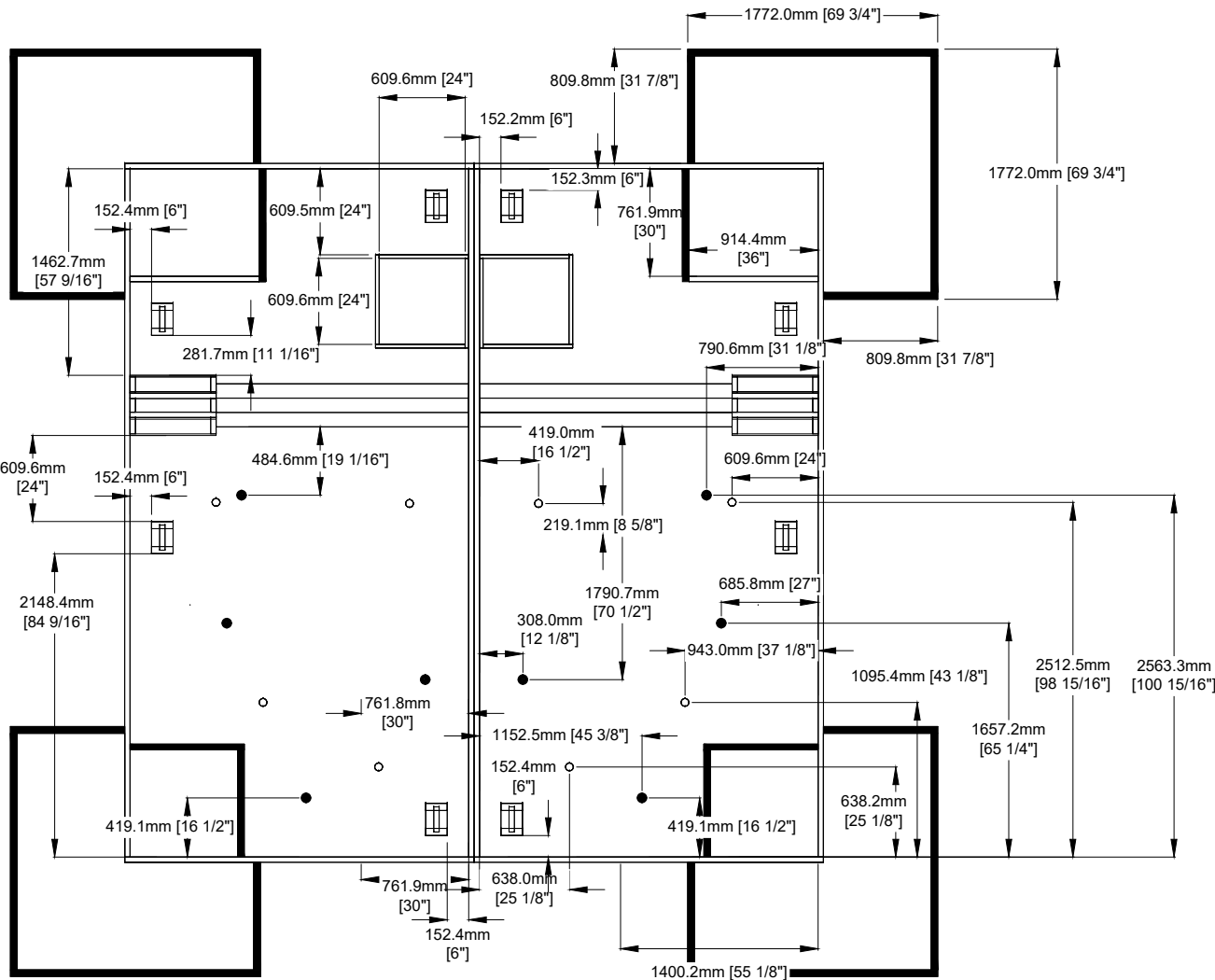
1 MAIN COURT DIMENSIONS (ROUND ROBIN AND TOURNAMENT LAYOUTS) SCALE = 1:50 (ON 8.5" x 11" PAPER)
