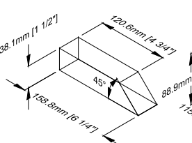
4 O DIMENSIONS SCALE = N/A
