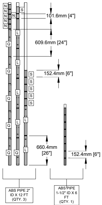
1 PIPE DETAILS SCALE = 1:50 (ON 8.5" x 11" PAPER)
